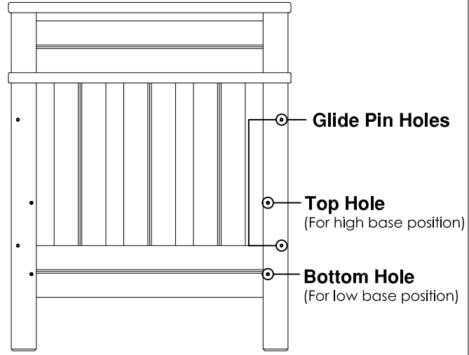
2 x End Panels (Identical)
